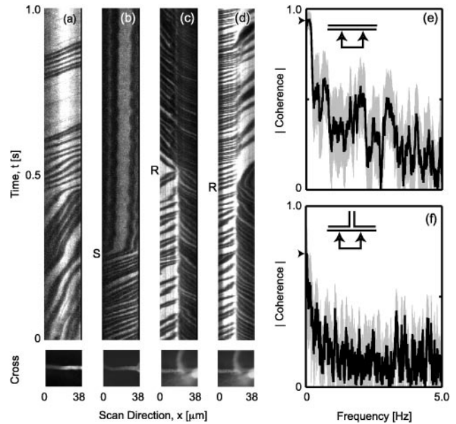
FIG. 4. Examples of highly variable flow. (a) A 1-sec segment of the line-scan data through a straight section of a capillary in which the speed changes from relatively slow (large slope) to fast (small slope). The image below the line-scan record is the average of 100 planar scans that include the axis of the capillary. Depth = 240 \mu\text{m} . (b) A 1-sec segment of data at the onset of a transient stall in flow (S). Note that the RBCs remain stuck in the vessel. Depth = 260 \mu\text{m} . (c) A 1-sec segment of data that shows the flow in two collinear arms of a junction. Note the reversal in the direction of flow in the arm on the left (R). Depth = 260 \mu\text{m} . (d) Segment of flow in the same capillary junction as in c acquired approximately 200 sec later. Multiple reversals in the direction of flow in the right arm were seen, one of which is shown (R). (e) Trial-averaged ( n = 8 ) spectral coherence between two \approx 10\text{-}\mu\text{m} segments in a straight vessel separated by a center-to-center distance of 25 \mu\text{m} . The thick line is the magnitude of the mean coherence and the gray band indicates one SD in the trial average ( n = 8 ). The arrow indicates the coherence at zero frequency. We used multitaper spectral estimation techniques (36) with a half-bandwidth of 0.04 Hz; the SD is a jackknife estimate (37). (f) Trial-averaged ( n = 4 ) spectral coherence between the velocity in right versus left arms of the junction shown in c and d .
