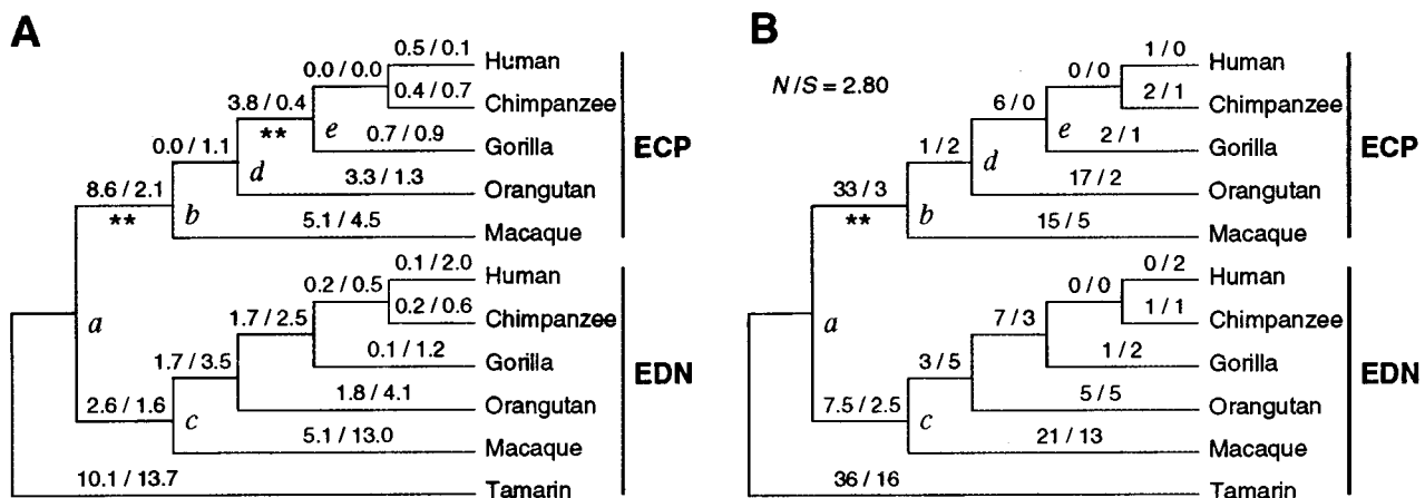
FIG. 1. Evolutionary tree of primate ECP and EDN genes. The root of this tree is located on the branch linking node a and the NW monkey tamarin if we use mouse sequences (54, 55) as outgroups. The gene duplication occurred at node a . (A) The \hat{b}_N and \hat{b}_S for each branch are presented as \hat{b}_N (\times 100) / \hat{b}_S (\times 100) above the branch. The standard errors of \hat{b}_N and \hat{b}_S are 0.0176 and 0.0151 for the branch a-b and 0.0108 and 0.0056 for the branch d-e , respectively. The statistical significance of the positiveness of \hat{b}_N - \hat{b}_S was determined by one-tailed Z test and is indicated by asterisks (**, 1%). (B) The numbers of nonsynonymous ( n ) and synonymous ( s ) substitutions per sequence per branch are presented as n/s above each branch. The N/S ratio for the sequences is given above the tree. The statistical significance of the difference between n/s and N/S was tested by Fisher's exact test (Table 1).
