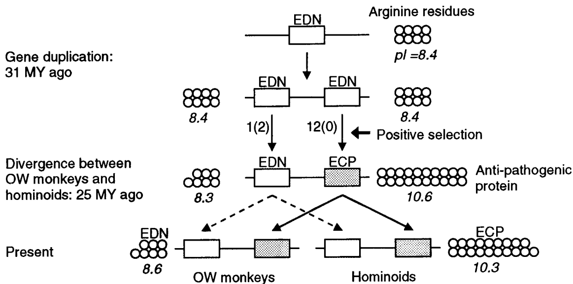
FIG. 3. Evolution of the novel anti-pathogen toxicity and arginine changes in ECP. Each circle represents one arginine residue in ECP or EDN sequences (see Fig. 2). For the present-day proteins, only the numbers of arginines for human sequences are presented. The average number of arginines for OW monkeys and hominoids is 18.2 for ECP and 7.6 for EDN. The pI value for each protein is also presented. The numbers of amino acid changes to arginines in the branches a-b and a-c in Fig. 1 are given alongside the arrow signs. The numbers of changes from arginines to other amino acids are given in parentheses. MY, million years.
