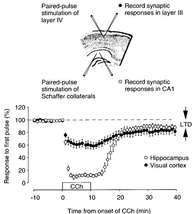
FIG. 1. A potential mechanism for the facilitation of LTD by novelty. Manahan-Vaughan and Brauneuwel (1) report that exposing a rat to a novel environment produces a striking facilitation of homosynaptic LTD in vivo . Similar to the effect of novelty exposure, transient application of carbachol, an analogue of ACh, enables induction of LTD in visual cortex and hippocampus by synaptic stimulation that is normally without effect. This figure is modified, with permission, from ref. 20.
