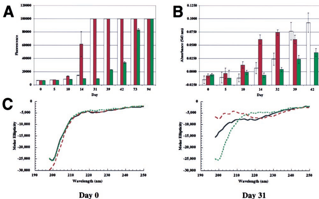
Fig. 1. Fibrillization and \beta -sheet formation of WT, A53T, and A30P \alpha -synuclein ( 300 \mu\text{M} ), followed by three complementary methods. (A) Thio T fluorescence assay shows that A53T fibrillizes most rapidly (red), followed by WT (white) and then A30P (green); signal of 100,000 is maximum (refer to Materials and Methods ). (B) Congo red-binding assay also shows that A53T fibrillizes most rapidly (red), followed by WT (white) and then A30P (green). (C) CD spectroscopy detects the random-coil (monomer)-to- \beta -sheet (fibril) transition. At day 0, all three variants are predominantly random coil. At day 31, the transition to \beta -sheet structure is most complete in the case of A53T (red), less in the case of WT (black), and has not begun in the case of A30P (green).
