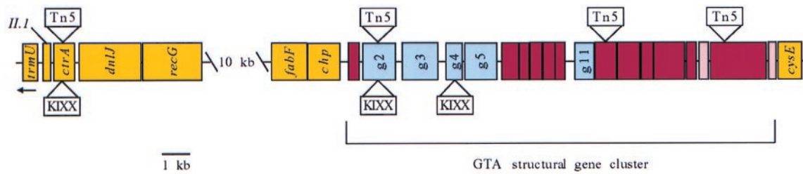
Fig. 1. Map of a region of the R. capsulatus chromosome containing genes necessary for GTA production. Locations of Tn5 and KIXX cartridge insertion found to abolish GTA production are shown. All ORFs are predicted to be transcribed left to right except for trmU . ORFs with weak or no similarity to known genes are shown in red or pink; ORFs homologous to known phage genes are shown in light blue; ORFs highly homologous to known cellular genes are shown in yellow. All predicted ORFs match R. capsulatus codon usage well, as defined by the highly expressed photosynthesis genes, except for those shown in pink ( orf17 and orf19 ). More detailed information about sequence similarities is given in Table 1. Information about the sources of the DNA sequences used to construct this figure is in the Results section.
