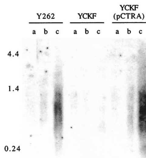
Fig. 5. RNA blot analysis of GTA gene transcripts. RNA was isolated from the strains indicated above the lines at three time points over the growth cycle: a, b, and c represent mid-log, late-log, and early stationary phases, respectively. Equal amounts (10 \mu g) of RNA were loaded in each lane. Approximate locations of molecular weight RNA standards are shown on the left (in kb). (A) Results when the blot was probed with a fragment of ctrA . (B) Results when the blot was probed with a fragment of orfg2 .
