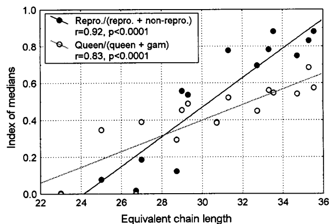
Fig. 4. Comparison of 15 compound peaks (see Table 1) that were present in reproductive queens and gamergates and nonlaying individuals. The equivalent chain length was correlated with a relative peak index (see Methods ), which represents the relative amount of the compounds in the respective group. The strong correlations suggest that the hydrocarbons are elongated with increasing ovarian activity.
