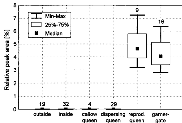
Fig. 1. Qualitative difference in the presence of 13,23-dimethylheptatriacontane between reproductives and nonreproductive individuals. Gamergates and reproductive queens are characterized by the presence of this long-chained dimethylbranched alkane.
