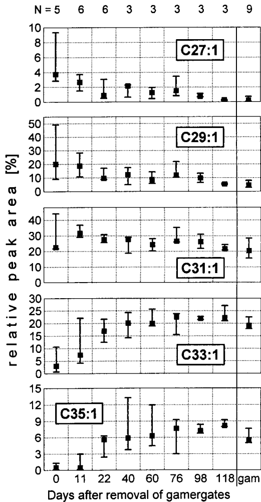
Fig. 5. The relative change of alkenes in the cuticular hydrocarbon profiles of new egg-laying workers after orphanage of the colony. At day 40, the sample size decreased to 3 because of the three workers that lost their rank at that time and were therefore excluded. For comparison, the relative amounts for the gamergates ( n = 9 ) that were laying eggs for more than six months were given in the column "gam." The short-chained alkenes show an inverse trend to the larger alkenes.
