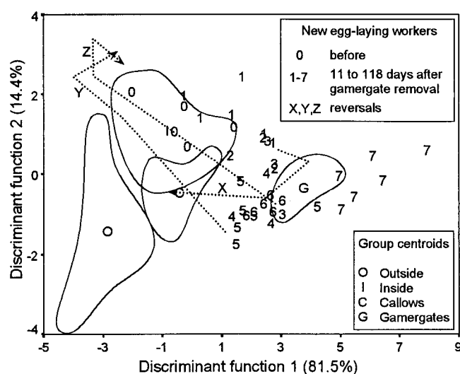
Fig. 3. The change of the hydrocarbon profiles of individuals that activated their ovaries. The discriminant analysis includes all members of colony A classified in four worker groups (gamergates, n = 9 ; callows, n = 9 ; workers from inside, n = 15 ; and from outside, n = 6 ). The differences in the CHC profiles of worker groups are illustrated by the respective encirclements based on the position of the individual group members similar to Fig. 2. Group centroids are marked. The change in the CHC profiles of those workers that started egg-laying after gamergate removal (new egg-laying workers) is indicated by numbers, which represent subsequent sampling periods (for respective sample days and size see Fig. 5). The change of the profiles of three workers that lost their rank ("reversals") is indicated by dotted lines, whereas the arrows show the directions (worker X sampled at days 48, 52, 58, and 67; Y at days 46, 56, 66, and 74; Z at days 50, 60, 65, and 72).
