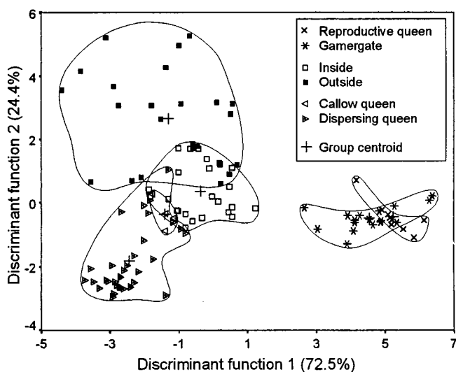
Fig. 2. Discriminant analysis of 6 groups of individuals from 13 colonies. Reproductive and nonreproductive individuals are separated completely (see Table 2) on the basis of the relative areas of 14 compound peaks indicated in Table 1. The groups are encircled arbitrarily.
