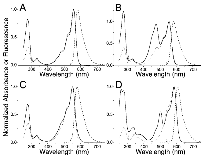
Fig. 3. Fluorescence and absorption spectra of DsRed (A), T1 (B), dimer2 and tdimer2(12) (C), and mRFP1 (D). The absorbance spectrum is shown with a solid line, the excitation with a dotted line, and the emission with a dashed line.
