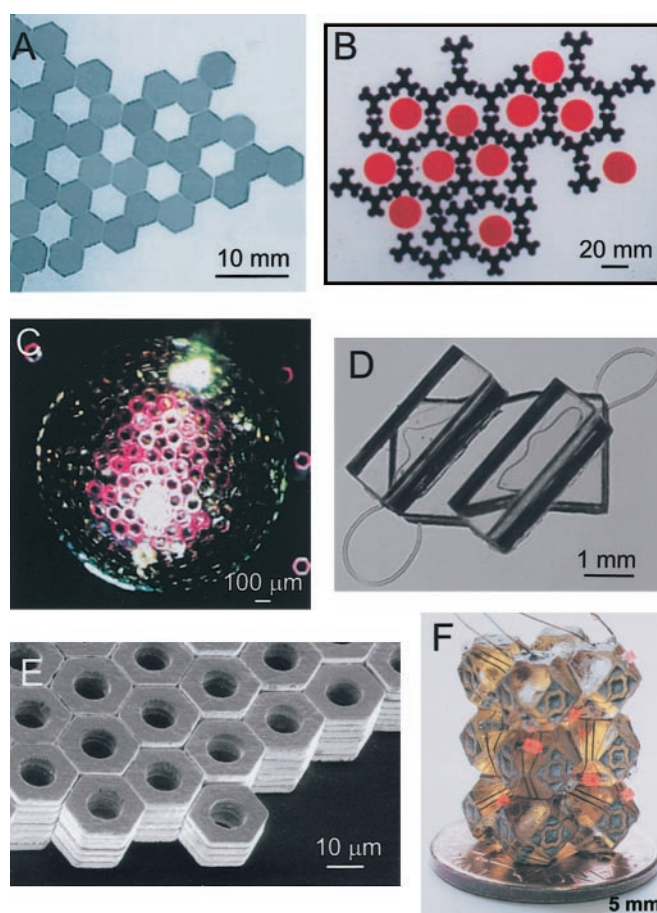
Fig. 2. Examples of two-dimensional (A and B) and 3D (C–F) structures, self-assembled in systems of macroscopic components interacting via capillary interactions. Open hexagonal array (A; reprinted with permission from ref. 33, copyright 1997 American Association for the Advancement of Science) and hexagonal lattice formed around circular templates (B; reprinted with permission from ref. 48, copyright 2000 American Chemical Society) self-assembled from poly(dimethylsiloxane) plates floating at the interface between perfluodecalin and water. (C) Spherical structure formed by self-assembly of hexagonal metal plates on the surface of a drop of perfluodecalin in water (reprinted with permission from ref. 49, copyright 1998 American Chemical Society). (D) Compact 3D structure formed by self-folding of a string of tethered, polymeric polyhedra (reprinted with permission from ref. 54, copyright 2002 American Chemical Society). (E) Large crystal self-assembled from micrometer-sized hexagonal metal plates (reprinted with permission from ref. 36, copyright 2001 American Chemical Society). (F) Aggregate with electrical connectivity self-assembled from polyhedral, polymer components bearing solder patterns of wires and dots (reprinted with permission from ref. 42, copyright 2000 American Association for the Advancement of Science).
