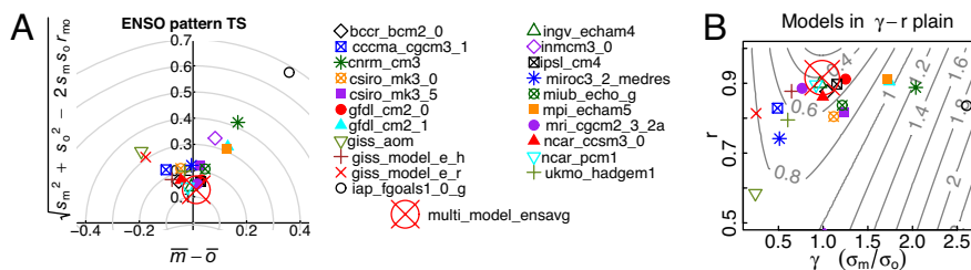
Fig. 4. Errors in the individual models and the multimodel ensemble average for one particular metric. (A) Shown is RMSE plot for the ENSO pattern in surface temperature (ts). (B) Shown is pattern error in ENSO ts ( y axis of A) decomposed into \gamma (the ratio of the standard deviation of the model to the observed) and r (the pattern correlation between the model and observed fields). Contours of the y axis value (the pattern error) from A are also shown on B; there is a minimum value of 0 located at (1, 1), and all values increase away from this minimum.
