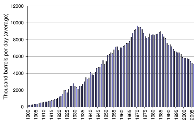
Fig. 2. Total annual US production of crude oil, 1900–2007. US production peaked in 1970 (14, 33).
