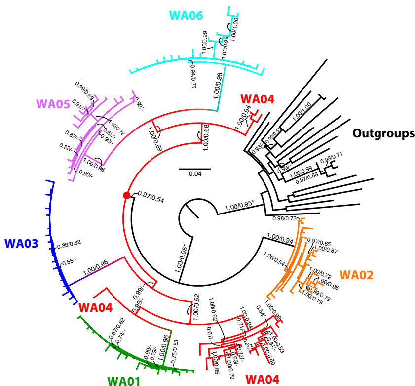
Fig. 2. Washington case: ML tree for the env gene dataset using BLAST-selected GenBank controls. Support values and clade coloring are as in Fig. 1. Color gradients along branches represent putative transmission events from WA04cd to other individuals.
