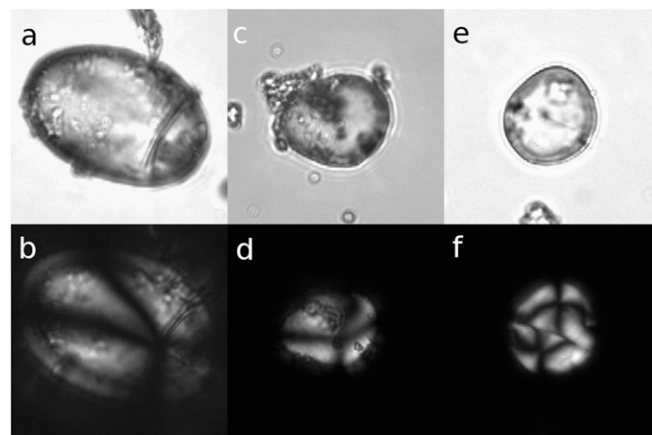
Fig. 4. Starch grains recovered from the calculus of Spy I and Spy II. The Upper image of each pair shows the starch under brightfield, and the Lower image shows it under cross-polarized light. Each box is 50 \mu\text{m} on a side. (A and B) Type 1, probable water lily starch. (C and D) Type 2. (E and F) Type 3.
