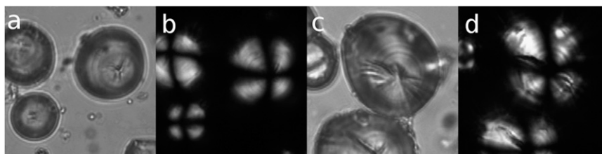
Fig. 5. Starch grains from modern water lilies under brightfield and cross-polarized light. Each box is 50 µm on a side. (A and B) Nymphaea alba . (C and D) Nuphar lutea .
