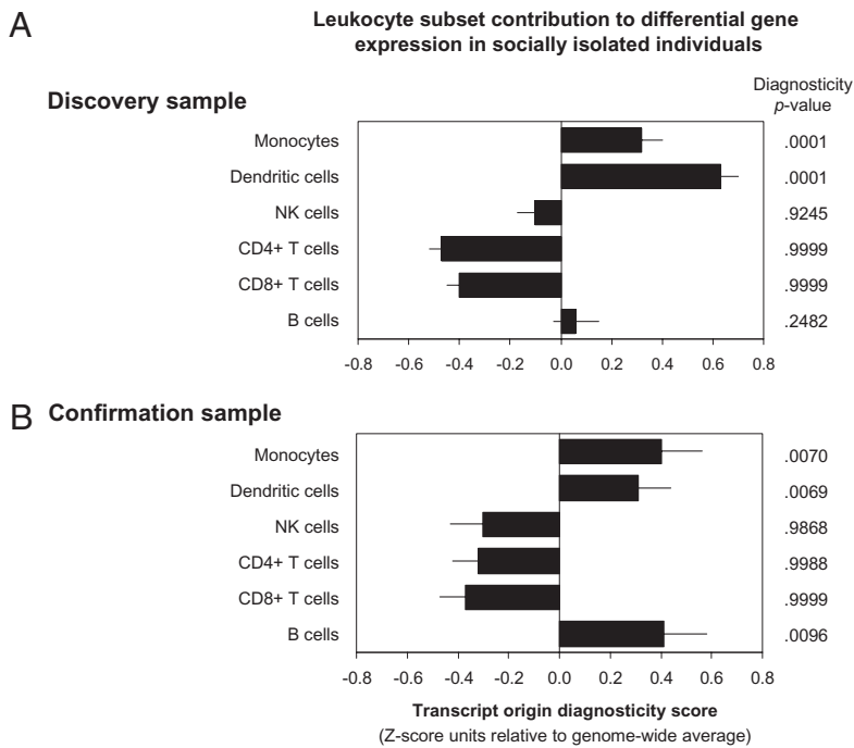
Fig. 1. Transcript origin analysis of genes differentially expressed in circulating leukocytes from chronically lonely vs. nonlonely individuals in a discovery sample of 14 individuals in study year 4 (A) and a confirmation sample of 93 individuals in study year 8 (B). Data represent mean \pm SE cell type diagnosticity score, with P values testing overrepresentation relative to the genome-wide null distribution for each cell type. Positive diagnosticity indicates that differentially expressed genes originate predominately from the analyzed cell type. Negative values are uninformative, implying that transcripts originate from other cell types or from the analyzed cell type as well as other cell types. Chronically lonely individuals were identified by UCLA Loneliness Scale scores in the top 15% of the sample distribution for each of the study's first 3 y (43% of the analyzed subsample) (A) or in the top quartile for 3 y or more of the study's first 5 y (26% of the analyzed sample) (B). All participants are healthy older adults enrolled in the CHASRS (4).
