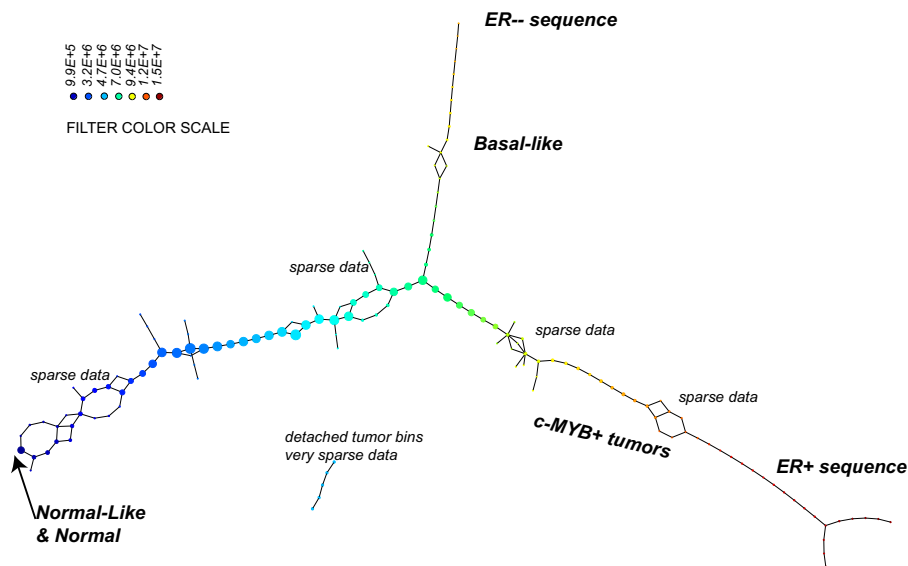
Fig. 3. PAD analysis of the NKI data. The output has three progression arms, because tumors (data points) are ordered by the magnitude of deviation from normal (the HSM ). Each bin is colored by the mean of the filter map on the points. Blue bins contain tumors whose total deviation from HSM is small (normal and Normal-like tumors). Red bins contain tumors whose deviation from HSM is large. The image of f was subdivided into 15 intervals with 80% overlap. All bins are seen (outliers included). Regions of sparse data show branching. Several bins are disconnected from the main graph. The ER^- arm consists mostly of Basal tumors. The c-MYB + group was chosen within the ER arm as the tightest subset, between the two sparse regions.
