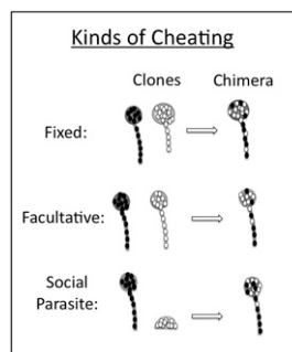
Fig. 3. In the social stage, clones may take advantage of their partner in three different ways. They may allocate cells to spore and stalk in the same proportions as alone but allocate less to stalk than their partner, fixed cheating. They may modify their behavior in chimera to take advantage of their partner, facultative cheating. Third, a social parasite can only make fruiting bodies in chimera with a victim.
