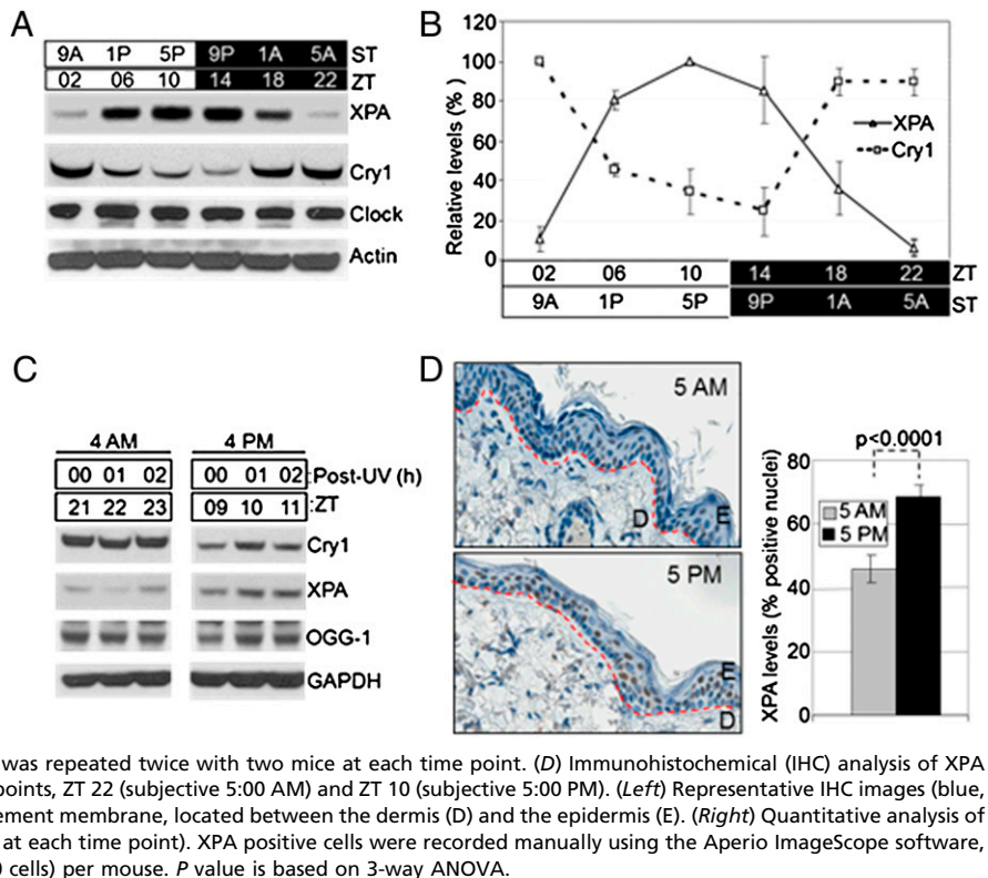
Fig. 1. Circadian oscillation of XPA in mouse skin. (A) Mice kept under an LD 12:12 cycle were killed at the indicated zeitgeber times (ZT 0 = light on) and the levels of the indicated proteins were determined from whole skin by immunoblotting. Light and dark boxes indicate the light-on and light-off phases, respectively. Note the robust and antiphase oscillations of the XPA and CRY1 proteins. The core clock protein, Clock, as expected (14), does not exhibit rhythmicity. Actin was used as a loading control. ST, subjective time, with light on at 7:00 AM and off at 7:00 PM. (B) Quantitative analysis of XPA and CRY1 oscillation in the mouse skin. Error bars represent means \pm SD ( n = 2 mice at each time point). (C) XPA expression in the epidermis of SKH-1 hairless mice. The mice were exposed to UVR at ZT 21 (subjective 4:00 AM) or ZT 9 (subjective 4:00 PM) and epidermis was harvested at 0, 1, 2, 4, 6, and 12 h postirradiation and analyzed for expression of the indicated proteins by immunoblotting. Note that XPA and CRY1 exhibit antiphase rhythms, whereas the oxidative base damage repair enzyme 8-oxo-guanine DNA glycosylase (OGG-1), implicated in repair of oxidative base damage caused by UVR, shows no rhythmicity. GAPDH is a loading control. A representative experiment is shown only with 0, 1, and 2 h postirradiation for clarity and both AM and PM samples were run on the same gel. This experiment was repeated twice with two mice at each time point. (D) Immunohistochemical (IHC) analysis of XPA expression in SKH-1 epidermis at two circadian time points, ZT 22 (subjective 5:00 AM) and ZT 10 (subjective 5:00 PM). (Left) Representative IHC images (blue, nuclei; brown, XPA). Red dashed lines follow the basement membrane, located between the dermis (D) and the epidermis (E). (Right) Quantitative analysis of IHC data. Error bars indicate means \pm SD ( n = 2 mice at each time point). XPA positive cells were recorded manually using the Aperio ImageScope software, counting at least 10 fields (each field consists of \sim 80 cells) per mouse. P value is based on 3-way ANOVA.
