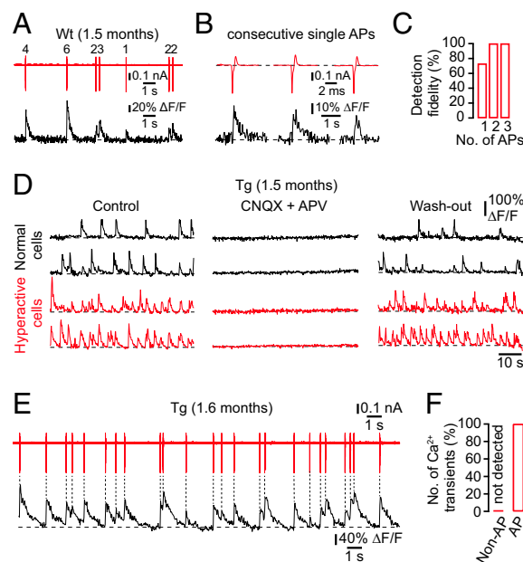
Fig. 3. Cellular mechanisms of spontaneous Ca 2+ transients in wild-type and transgenic mice. (A) Simultaneous in vivo recordings of spontaneous Ca 2+ transients (black trace) and underlying action potential (AP) firing (red trace; number of APs indicated) in a cell-attached configuration from a CA1 neuron in a wild-type mouse. (B) Examples of spontaneous Ca 2+ transients (black trace) evoked from three consecutive single APs (red trace) in a WT mouse. (C) Fractions of single APs and trains of APs optically detected in CA1 neurons of WT mice ( n = 15 cells in three mice). (D) Spontaneous Ca 2+ transients in normal (black traces) and hyperactive (red traces) CA1 neurons of a transgenic mouse before, during, and after local application of CNQX and APV. (E) Simultaneous in vivo recordings of spontaneous Ca 2+ transients (black trace) and underlying action potential firing (red trace) in a cell-attached configuration from a CA1 neuron in a tg mouse. (F) Number of spontaneous Ca 2+ transients triggered (AP) and not triggered (non-AP) by action potential firing in tg mice ( n = 13 cells in three mice).
