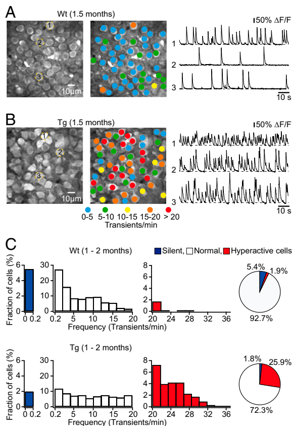
Fig. 2. Abnormal hyperactivity of hippocampal neurons in predisposing transgenic mice. (A and B) (Left) CA1 neurons imaged in vivo in a wild-type and a transgenic mouse, respectively. (Center) Activity maps, in which hue is determined by the frequency of spontaneous Ca 2+ transients, overlaid with the anatomical image (Left). (Right) Spontaneous Ca 2+ transients of the corresponding neurons marked (Left). (C) The frequency distribution of spontaneous Ca 2+ transients was shifted toward higher frequencies in tg (Lower; n = 818 cells in seven mice) compared with wild-type mice (Upper; n = 693 cells in six mice). Pie charts show the relative proportions of silent, normal, and hyperactive neurons.
