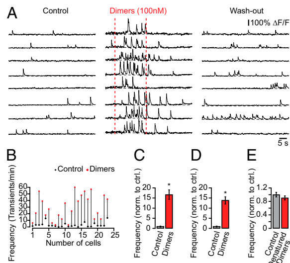
Fig. 5. Soluble A \beta induces hyperactivity in hippocampal neurons of wild-type mice. ( A ) Ca ^{2+} transients in CA1 neurons of a wild-type mouse before, during, and after local application of synthetic A \beta 526C dimer solution (30 s, 100 nM in the application pipette). ( B ) Rates of Ca ^{2+} transients in all recorded neurons from the experiment in A before (black) and during (red) dimer application. ( C ) Summary graph from the experiment in A showing the effect of dimers on the frequency of Ca ^{2+} transients (normalized to control, n = 24 cells; *P < 0.001 , Student's t test). ( D ) Summary graph from all experiments illustrating the effect of dimers on the frequency of Ca ^{2+} transients (normalized to control, n = 83 cells in three mice; *P < 0.001 , Student's t test). ( E ) Summary graph showing that heat-denatured dimers have no significant effect on the frequency of Ca ^{2+} transients (normalized to control, n = 158 cells in three mice; P > 0.05 , Student's t test). All error bars denote SEM.
