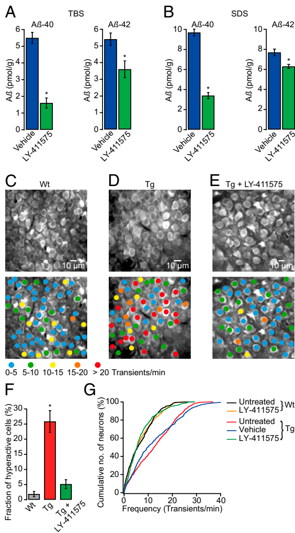
Fig. 4. A single dose of \gamma -secretase inhibitor reduces soluble A \beta levels and rescues neuronal dysfunction in transgenic mice. ( A and B ) Acute LY-411575 treatment significantly reduced TBS- and SDS-soluble A \beta -40 and A \beta -42 hippocampal levels in transgenic mice ( n = 4 –5 mice per group; *P < 0.001 for A \beta -40 and *P < 0.05 for A \beta -42, Student's t test). ( C–E ) ( Upper ) CA1 neurons imaged in vivo in a WT, a tg, and an LY-411575-treated tg mouse, respectively. ( Lower ) Activity maps, in which hue is determined by the frequency of spontaneous Ca ^{2+} transients, overlaid with the anatomical image ( Upper ). ( F ) The fraction of hyperactive neurons was significantly smaller in LY-411575-treated tg ( 5.13 \pm 1.47\% , n = 5 mice) than in untreated tg mice ( 25.85 \pm 3.59\% , n = 7 mice; *P < 0.001 , Student's t test) and not significantly different from untreated WT mice ( 1.85 \pm 0.86\% , n = 6 mice; P > 0.05 , Student's t test). ( G ) Cumulative distributions of spontaneous Ca ^{2+} transients in LY-411575-treated tg mice ( n = 709 cells) were not significantly different from untreated WT ( n = 693 cells) and LY-411575-treated WT controls ( n = 841 cells; P > 0.05 , Kolmogorov–Smirnov test), but they were significantly different from vehicle-treated tg ( n = 484 cells) and untreated tg mice ( n = 818 cells; *P < 0.001 , Kolmogorov–Smirnov test). All error bars denote SEM.
