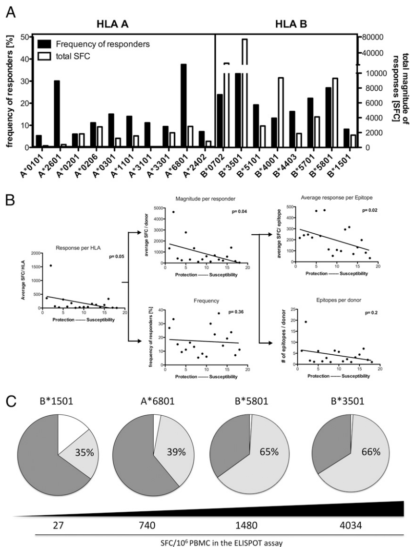
Fig. 4. HLA-linked T-cell responses. (A) Differential frequency and magnitude of HLA restricted responses in dengue-seropositive donors ( n = 182 ). Frequency (filled bars) and the magnitude (open bars) of T-cell responses (as total SFCs per 10^6 PBMC values) sorted according to their restriction element are shown. (B) Association of HLA restricted T-cell responses with disease susceptibility. Disease susceptibility was correlated with the average magnitudes of HLA restricted responses (Left), with the frequency and the magnitude of T-cell responses per donor (Center) and with the magnitude per epitope as well as breadth of response (Right). One-tailed Spearman test was then used to calculate correlations. The best positive correlation was observed with the magnitude of response per epitope ( P = 0.02 ). (C) Multifunctionality of HLA restricted responses. Representative donors were stimulated with HLA restricted donor-specific peptide pools for 6 h in the presence of BFA. Cells were then stained with mAb against surface markers CD3 and CD8 and mAb against intracellular IFN\gamma , TNF\alpha , and IL2. Pie charts represent cytokine profiles of individual donors. The relative number of cells producing one (dark gray areas), two (light gray areas), or three (white areas) of the measured cytokines is shown. Percentages in the pie charts represent the relative number of cells that produce two or more cytokines. Numbers under the pie charts represent the T-cell responses (as IFN\gamma SFCs per 10^6 PBMCs) of this specific donor/allele combination in the ELISPOT assay ( n = 4 ).
