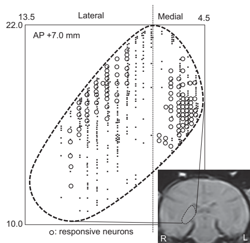
Fig. 3. Stereotaxic plots of the pulvinar neurons on the MRI photo of the monkey brain. The 745 pulvinar neurons were recorded from AP 8.0 to AP 5.0, but plotted on the plane at AP 7.0. The number in the left upper corner indicates the distance (in millimeters) anteriorly from the interaural line. The horizontal axis indicates the distance (in millimeters) from the midline; vertical axis indicates the distance (in millimeters) from the interaural line. Open circles, visually responsive neurons; dots, nonresponsive neurons.
