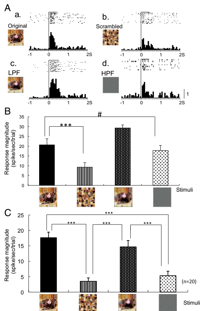
Fig. 4. Effects of scrambling and filtering of the images. (A) An example of neuronal responses to the original ( a ), scrambled ( b ), and filtered [ c (LPF), d (HPF)] images (same neuron shown in Fig. 1). (B) Response magnitudes to the stimuli shown in A . Scrambling significantly decreased (***Tukey test after one-way ANOVA, P < 0.001 ) and HPF tended to decrease the responses to the original image (Tukey test after one-way ANOVA, P < 0.10 ). (C) Mean response magnitudes to the scrambled and filtered images ( n = 20 ). Scrambling and HPF significantly decreased the responses to the original image (***Tukey test after one-way ANOVA, P < 0.001 ).
