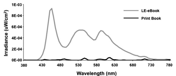
Fig. 4. Spectral radiometric profile of the LE-eBook device (gray) and incident light reflected by the printed book (black). The peak irradiance for the LE-eBook eReader is \sim 450 nm and for the reflected light is 612 nm.
