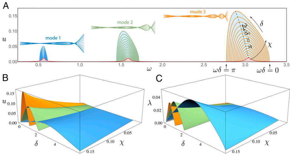
Fig. 3. Proprioceptive swimming. (A) Families of self-propelled feedback-driven solutions as functions of \delta and \chi , in the proximity of the natural resonance frequencies (passive sheet, red line), obtained by solving Eqs. 15–17 with m_a \neq 0 (Eq. 9), m_a = 0 , \rho_f = \rho_s = 1,000 \text{ kg/m}^3 , Re^b = 3.5 \cdot 10^4 , \rho = 300 . For each resonance peak, a representative proprioceptive swimmer's midline trace is reported. (B) The locomotion velocity u and (C) the tail amplitude \lambda as functions of \delta and \chi . In A–C the blue, green, and orange surfaces are associated with the first, second, and third resonance peak. The maximum velocity and tail amplitude are located at \omega\delta = \pi/2 .
