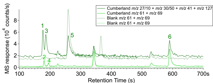
Fig. 2. GC chromatograms of CB-5 sample with m/z corresponding to the base or diagnostic peak of each of the N-bearing compounds identified. 1, NO ( m/z 30); 2, TFA ( m/z 69); 3, HCN ( m/z 27); 4, C1CN ( m/z 61); 5, CH 3 CN ( m/z 41); 6, TFMA ( m/z 127). Division factors were applied to the most abundant compounds for scaling: factor 10 for m/z 27 and factor 50 for m/z 30. None of the chosen masses contribute to another N-bearing compound identified in each chromatogram. Because of partial coelutions between the first four GC peaks, two separate chromatograms were reconstructed (dark green and light green plain lines). The corresponding dotted lines are the reconstructed chromatograms of the reheated CB-6-residue sample, which has the same GC temperature cut as CB-5 and can thus be considered as a blank. Although acetonitrile (CH 3 CN) ( m/z 41) is detected in the GC, its detection in EGA is complicated by methylpropene, which constitutes the majority of the signal at m/z 41.
