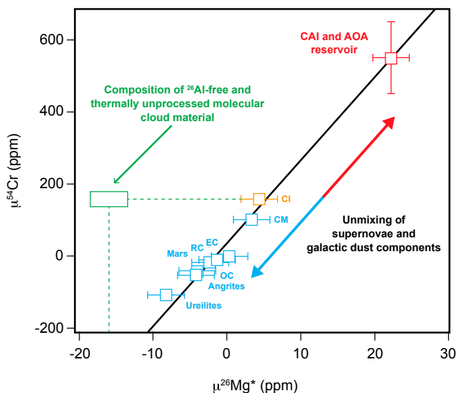
Fig. 1. Inner Solar System \mu^{26}\text{Mg}^* - \mu^{54}\text{Cr} correlation. The \mu -notation reflects the deviation in parts per millions (ppm) of the internally normalized ^{26}\text{Mg}/^{24}\text{Mg} and ^{54}\text{Cr}/^{52}\text{Cr} ratios from the terrestrial compositions. Uncertainties reflect the external reproducibility or internal errors, whichever is larger. The \mu^{54}\text{Cr} uncertainties are typically smaller than symbols. AOA, amoeboid olivine aggregates; EC, enstatite chondrites; OC, ordinary chondrites; RC, Rumuruti chondrites. Data are from ref. 13 and this study. The \mu^{54}\text{Cr} and \mu^{26}\text{Mg}^* compositions of the ^{26}\text{Al} -free and thermally unprocessed molecular cloud material, including their uncertainties, are defined by CI chondrites and the initial \mu^{26}\text{Mg}^* value of the Solar System (13). AOA and CAls represented here are objects that formed with the canonical ^{26}\text{Al}/^{27}\text{Al} of \sim 5 \times 10^{-5} . Although CI chondrites are commonly viewed as reflecting the bulk Solar System composition for most elements, it is unclear whether this assumption is correct for the \mu^{26}\text{Mg}^* and \mu^{54}\text{Cr} values. This can be tested through high-precision Mg and Cr isotope measurements of the Sun, which is currently not possible at a level of precision relevant to our discussion. See SI Appendix, Fig. S8 , for additional information with respect to the end-member compositions considered in the model.
