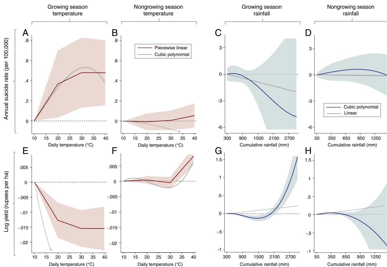
Fig. 1. Nonlinear relationships between temperature, precipitation, suicide rates, and crop yield: The response of annual suicides rates (deaths per 100,000 people) to (A) growing season and (B) nongrowing season temperatures. Response of annual suicide rates to cumulative (C) growing season and (D) nongrowing season rainfall. (E–H) Analogous relationships for log annual yield, valued in rupees per hectare. The slopes of the responses in A, B, E, and F can be interpreted as the change in the annual suicide rate or log yield caused by one day's temperature rising by 1 °C. The slopes of the responses in C, D, G, and H can be interpreted as the change in the annual suicide rate or log yield caused by one additional millimeter of rainfall. All graphs are centered at zero.
