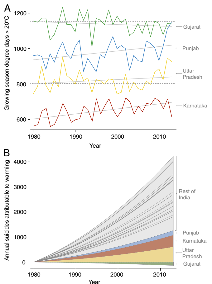
Fig. 4. Attribution of suicides to warming trends in growing season temperatures since 1980: (A) trends in degree days above 20 °C during India's main growing season for four example states and (B) the total number of deaths annually that can be attributed to warming trends, using the estimated marginal effects of degree days on suicide rates.
