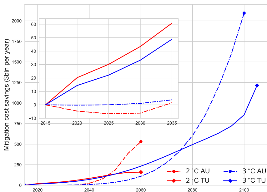
Fig. 2. Mitigation cost savings from moving from the UN-medium to the UN-low population path, under TU and AU social objectives, given 2 °C and 3 °C temperature targets. Cost savings stop when full abatement is reached in both population scenarios.
