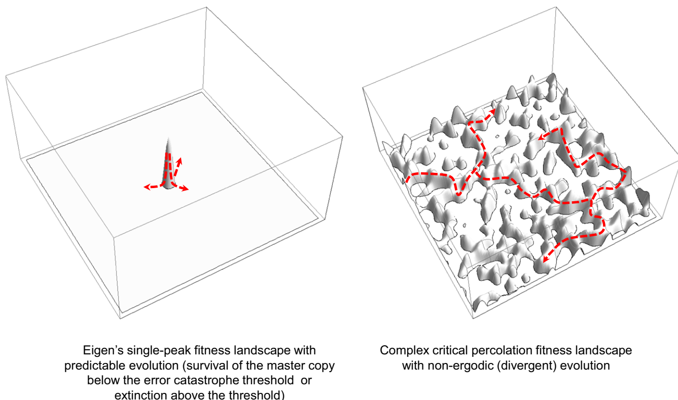
Fig. 2. Complexity of fitness landscapes and nonergodicity of evolution.
