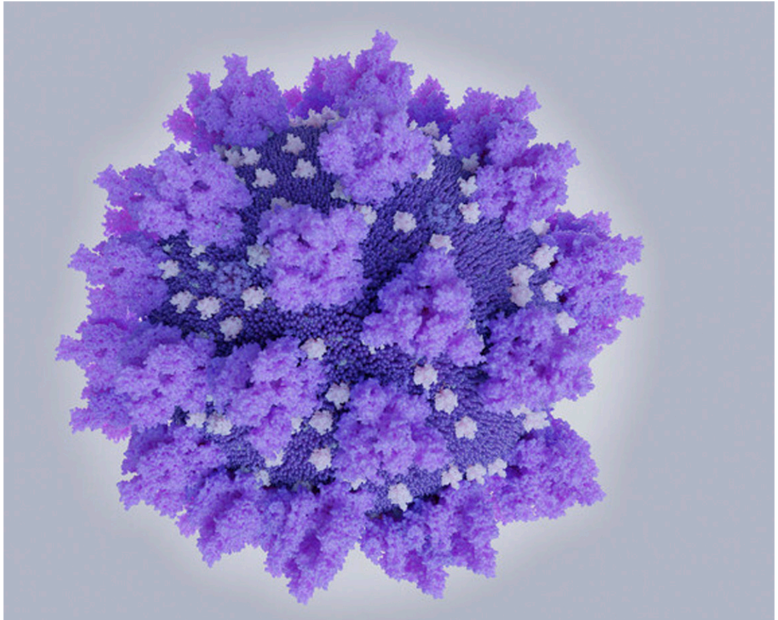
SARS-CoV-2—the virus that causes COVID-19 and the focus of numerous vaccine development efforts—has three surface proteins attached to a lipid bilayer, as seen in this illustration based on X-ray diffraction data. Image credit: Science Source/Juan Gaertner.
