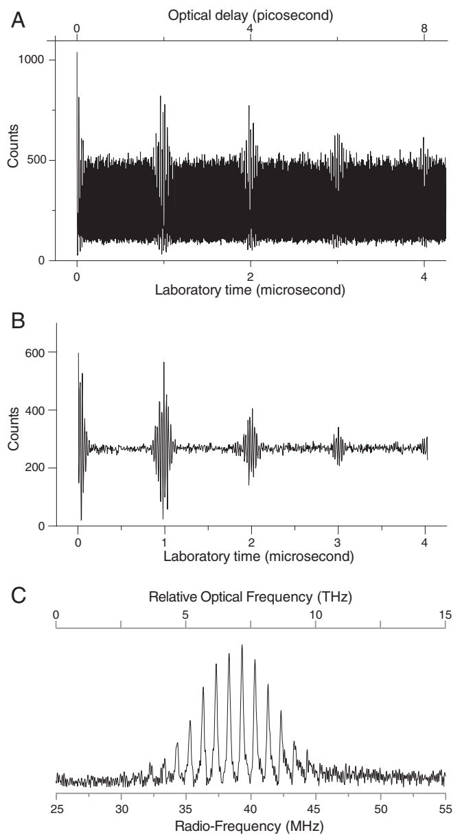
Fig. 2. Experimental dual-comb interferogram and spectrum at a detected photon rate 2.7 \times 10^6 photons per \text{s}^{-1} . (A) The raw interferogram sampled at a rate of 0.8 ns (lower x scale: laboratory time) comprises a background part, unmodulated by the interference. The periodic interference signatures of a Fabry-Pérot étalon appear with a high contrast even at an optical delay of 8 ps (upper x scale: optical delays). (B) The interferogram of A is numerically filtered to highlight better the photon-counting interference signal. (C) The Fourier transform of a photon-counting interferogram (including A) reveals the evenly spaced transmission lines of the étalon, over a broad spectral span of several terahertz in the optical domain.
