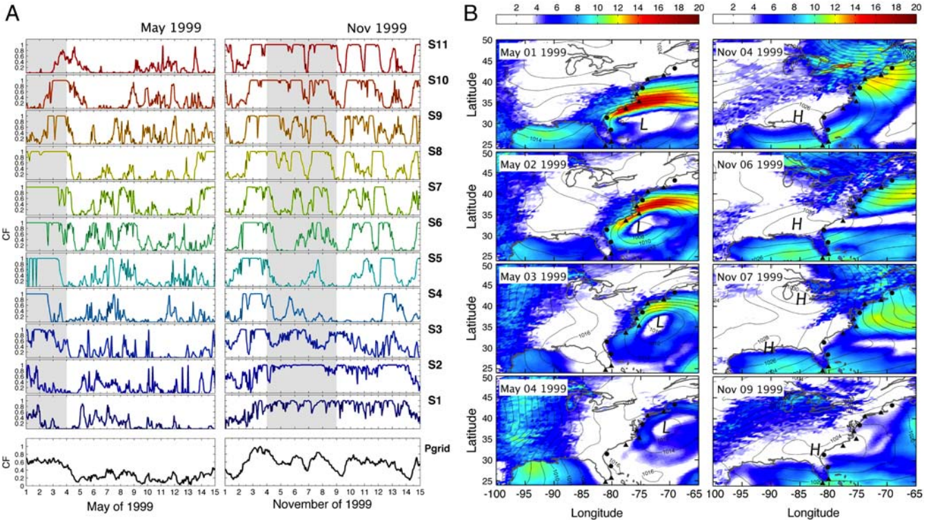
Fig. 6. (A) Capacity factors for 11 stations in May 1999 and November 1999; line colors match station colors in Fig 1. The lowest graph, P_{\text{grid}} , is the aggregate CF if all stations are connected by transmission. The two gray date ranges are each expanded to 4 d on the maps (B). (B) Sea level pressure (lines, in hPa) and wind speed (color scale at top, in \text{m s}^{-1} ) for the events from May 1–4 (Left) and November 4–9 (Right), 1999.
