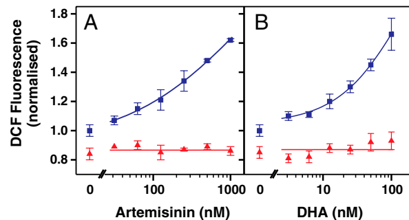
Fig. 5. Artemisinin (A) and DHA (B) exert prooxidant activity that is antagonized by inhibition of hemoglobin digestion. Trophozoite stage parasites (2% hematocrit, 1% parasitemia) labeled with CM-H 2 DCFDA were incubated for 1 h in the absence (blue squares) or presence (red triangles) of 5 \mu M ALLN before an additional 2 h incubation with artemisinin or DHA. The cells were washed and the median DCF signal of the parasite population analyzed by flow cytometry. Data are normalized to untreated controls (no endoperoxide or inhibitor). Error bars represent SD of triplicate measurements.
