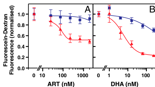
Fig. 3. RBC lysate is needed for artemisinin (A) or DHA (B)-mediated inhibition of endocytosis. Mid trophozoite stage parasites were released from RBCs with 0.02% (w/v) saponin and incubated for 4 h with fluorescein-dextran in the absence (blue squares) and presence (red triangles) of RBC lysate containing 3.7 mM hemoglobin. The median green fluorescence signal of the parasite population was used as a measure of uptake. Error bars represent SD of triplicate measurements.
