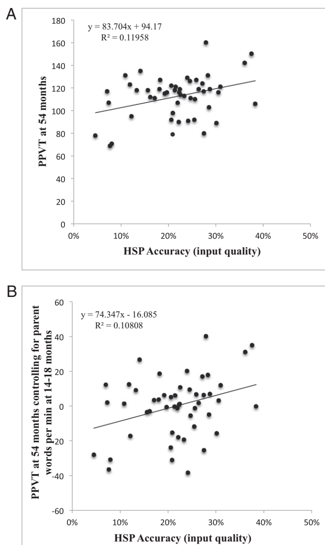
Fig. 1. Effect of quality of early input at 14–18 mo on child comprehension vocabulary at 54 mo. ( A ) Quality of word learning instances (average HSP accuracy per family) at 14–18 mo predicts child comprehension vocabulary (PPVT) at 54 mo. ( B ) This effect holds even after controlling for the quantity of early input (average parent words per minute at 14 and 18 mo). Each point represents a single family ( n = 50 ).
