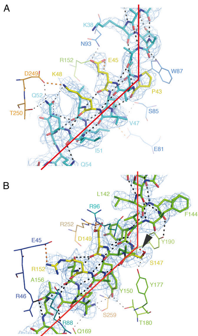
Fig. 3. Proline and serine residues in the signature motifs of Aac2p. (A) The signature motif of H1 (cyan) and (B) of H3 (green) of Aac2p (chain A of P2 1 2 1 ). Residues interacting with the side-chains are shown in line representation. Residues of the signature motif are shown in yellow. Hydrogen bonds involving backbone atoms are shown as thick black-dotted lines, hydrogen bonds not involving backbone atoms are shown as thin black-dotted lines. Salt bridges are shown as orange-dotted lines. The density, shown as a blue mesh, is a 2mF_o - DF_c map, contoured at 1 \sigma , and displayed within 2 \text{ \AA} of the atoms. In B, the unusual hydrogen bond from the side-chain of Ser147 to its own backbone amide is highlighted in red dots, and indicated by an arrowhead.
