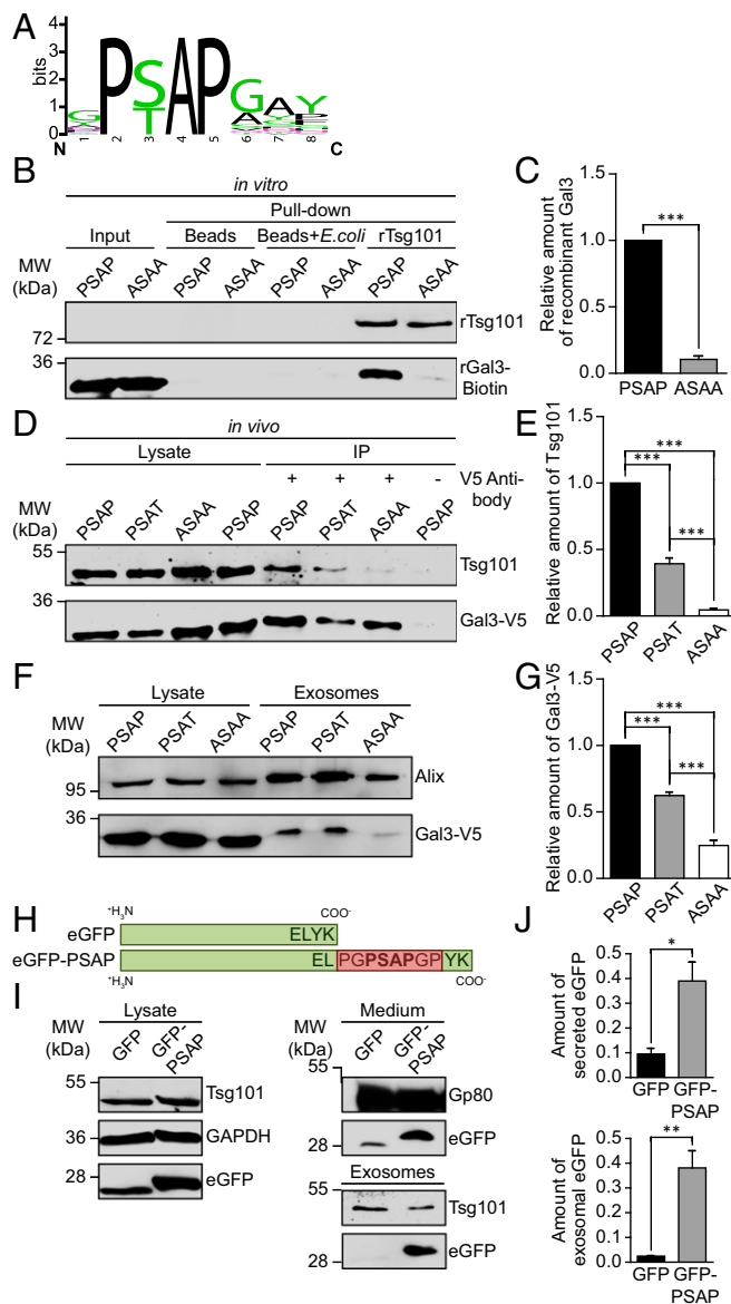
Fig. 6. The PSAP domain of Gal3 is responsible for the interaction with Tsg101 and required for exosomal secretion. (A) An alignment of Gal3 late domain-like motifs found in 34 vertebrates was used to generate a sequence logo of the octapeptide (94)QPSAPGAY(101) ( SI Appendix, Fig. S8 ). (B) In vitro pull-down assay with recombinant Gal3 mutants and Tsg101-GST [PSAP, human recombinant Gal3, labeled with biotin; ASAA, human recombinant Gal3 with a mutated late domain-like motif (95)PSAP(98)→(95)ASAA(98), labeled with biotin; rTsg101, recombinant human Tsg101]. Negative controls: beads only; beads which were incubated with Escherichia coli lysate. (C) Quantification of experiments as in B, normalized to input. Means \pm SEM, n = 3 independent experiments. (D) Coimmunoprecipitation of Gal3-V5 mutants in MDCK cells [PSAT, human Gal3-V5 with a mutated late domain-like motif (95)PSAP(98)→(95)PSAT(98), which is a natural variant in humans]. (E) Quantification of experiments as in D. Negative control, Gal3-V5-PSAP lysate without anti-V5 antibody. Normalized to the respective cell lysate. Means \pm SEM, n = 3 independent experiments. (F) Immunoblot analysis of exosomal fractions in the Gal3-V5 mutants. (G) Quantification of experiments as in F. Normalized to the respective cell lysate. Means \pm SEM, n = 6 independent experiments. (H) Schematic drawing of the eGFP-PSAP polypeptide in comparison with eGFP. (I) At 48 h following transient transfection, cell culture media from MDCK cells expressing eGFP or eGFP-PSAP were collected to purify exosomes. Cell lysates, media, and isolated exosomes were analyzed by immunoblot. (J) Quantification of experiments as in I. Normalized to eGFP or eGFP-PSAP levels in the respective cell lysate. Means \pm SEM, n = 3 independent experiments. Statistical analysis: Student's unpaired t test, ***P < 0.001 , **P < 0.01 , *P < 0.05 .
