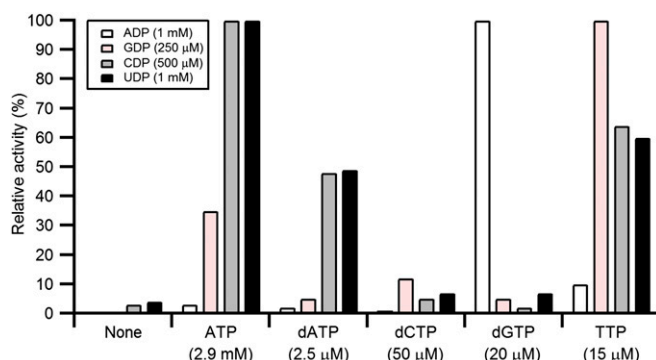
Fig. 2. Allosteric regulation of B. subtilis RNR substrate specificity using Mn(III) 2 -Y-NrdF and aiNrdE (described subsequently). Activities are expressed as a percentage relative to the maximum activity observed for a given substrate. Maximum activities for S (E) in \alpha_2\beta_2 are ADP (dGTP) = 420 \pm 20 \text{ nmol}\cdot\text{min}^{-1}\cdot\text{mg}^{-1} , GDP (TTP) = 245 \pm 10 \text{ nmol}\cdot\text{min}^{-1}\cdot\text{mg}^{-1} , CDP (ATP) = 385 \pm 20 \text{ nmol}\cdot\text{min}^{-1}\cdot\text{mg}^{-1} , and UDP (ATP) = 435 \pm 12 \text{ nmol}\cdot\text{min}^{-1}\cdot\text{mg}^{-1} . Assays (500 \mu\text{L} ) were conducted at 37 ^\circ\text{C} and contained a 1:1 mixture of 0.5- \mu\text{M} His 6 -tagged subunits, the endogenous reducing system (40- \mu\text{M} TrxA, 0.4- \mu\text{M} TrxB, and 0.2-mM NADPH), and S and E nucleotides at the concentrations indicated in the figure.
