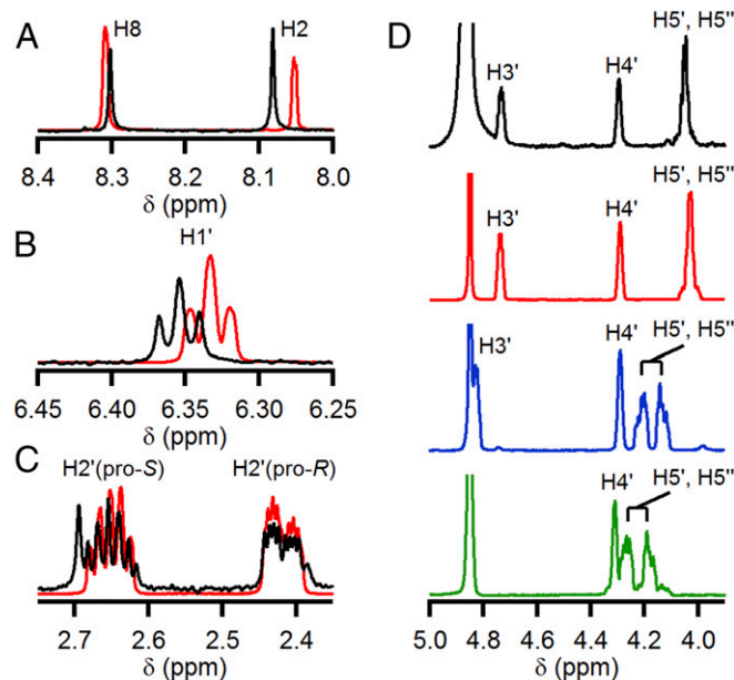
Fig. 3. Comparison of ^1\text{H-NMR} spectra of the deoxynucleoside monophosphate recovered from aiNrdE (black trace) with authentic dAMP (red trace), dADP (blue trace), and dATP (green trace) standards. The panels show regions of the spectra containing peaks that correspond to protons associated with the adenine base (A), the anomeric carbon (C1') (B), the 2' carbon (C), and carbons C3', C4', and C5' (D). Note that H3' for dATP is masked by the \text{H}_2\text{O}/\text{DOH} solvent peak.
