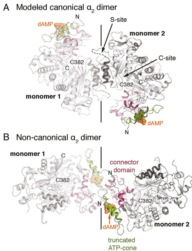
Fig. 1. Comparison of the modeled canonical and noncanonical dimeric forms of B. subtilis NrdE. (A) A model of the canonical dimer was generated via secondary-structure matching structural superposition (1) of the dAMP-bound B. subtilis NrdE monomer structure against the Salmonella typhimurium NrdE \alpha_2 dimer (PDB ID code 1PEM) (2). Disordered S-site residues are shown as dashed lines. (B) Crystal structure of the noncanonical dimer of dAMP-bound B. subtilis NrdE at pH 4. In both panels, the dimer interface is indicated by a solid black line. The N-terminal partial cone (green), the connector region (pink), and the two helices at the S-site in the canonical NrdE dimer (dark gray) are colored by domain. These colors are used throughout this report.
