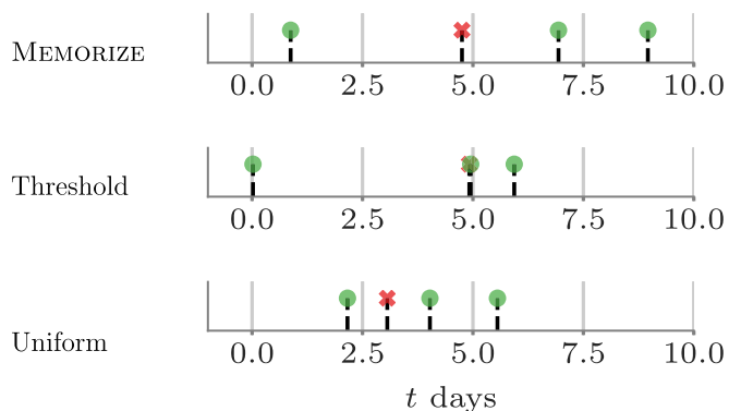
Fig. 1. Examples of (user, item) pairs whose corresponding reviewing times have high likelihood under MEMORIZE (Top), threshold-based reviewing schedule (Middle), and uniform reviewing schedule (Bottom). In every plot, each candlestick corresponds to a reviewing event with a green circle (red cross) if the recall was successful (unsuccessful), and time t = 0 corresponds to the first time the user is exposed to the item in our dataset, which may or may not correspond with the first reviewing event. The pairs whose reviewing times follow more closely MEMORIZE or the threshold-based schedule tend to increase the time interval between reviews every time a recall is successful while, in contrast, the uniform reviewing schedule does not. MEMORIZE tends to space the reviews more than the threshold-based schedule, achieving the same recall pattern with less effort.
