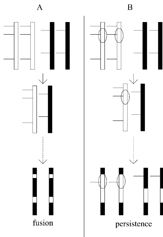
Fig. 2. Model for the long term effect of inversions on introgression and species persistence with hybridization. Two species are designated by diploid chromosomes of a single color (black or white) at the top of the figure. Horizontal lines indicate the locations of alleles that confer hybrid sterility in a heterospecific genetic background. The oval indicates an inverted gene arrangement relative to the other species. (A) No inversion difference between species. (B) One inversion differentiates the species.
