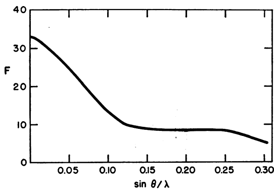
FIGURE 4 Calculated x-ray form factors for the pleated sheet, for planes parallel to the plane of the sheet.
