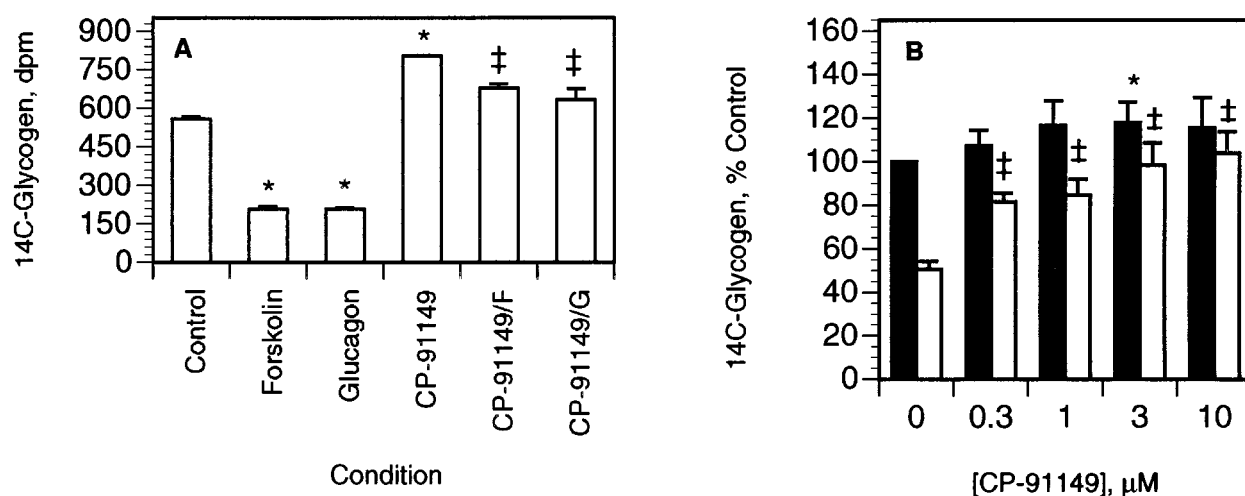
FIG. 6. Inhibition of glycogenolysis by CP-91149 in primary human hepatocytes. Primary human hepatocytes were incubated with [ ^{14}\text{C} -U]glucose plus 1 \mu\text{M} insulin, then with 10 mM glucose and (A) 50 \mu\text{M} forskolin (F) or 25 nM GGN (G), plus 30 \mu\text{M} CP-91149 as indicated, or (B) in the absence (filled bars) or presence (open bars) of 25 nM GGN, plus CP-91149 as indicated for 2 h. (A) Results (dpm ^{14}\text{C} -glycogen) are the mean \pm SEM of triplicate determinations from a representative experiment. *, P < 0.001 between GGN, forskolin, or CP-91149 vs. untreated control; ‡, P < 0.01 between control + GGN or forskolin vs. CP-91149 + GGN or forskolin. (B) Results are expressed relative (%) to untreated control in the absence of GGN (100%) and are the mean \pm SEM from 3 to 10 independent experiments, each performed in triplicate. *, P < 0.05 between CP-91149 vs. untreated control; ‡, P < 0.001 between CP-91149 + GGN vs. GGN-treated control.
