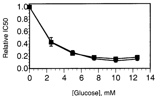
Fig. 3. The effect of glucose on the potency of CP-91149 (■) and caffeine (●). IC 50 values for HLGPa inhibition were determined at varied glucose concentrations, and then normalized by dividing the values by the IC 50 value obtained in the absence of glucose. The normalized results are plotted as function of glucose concentration.
